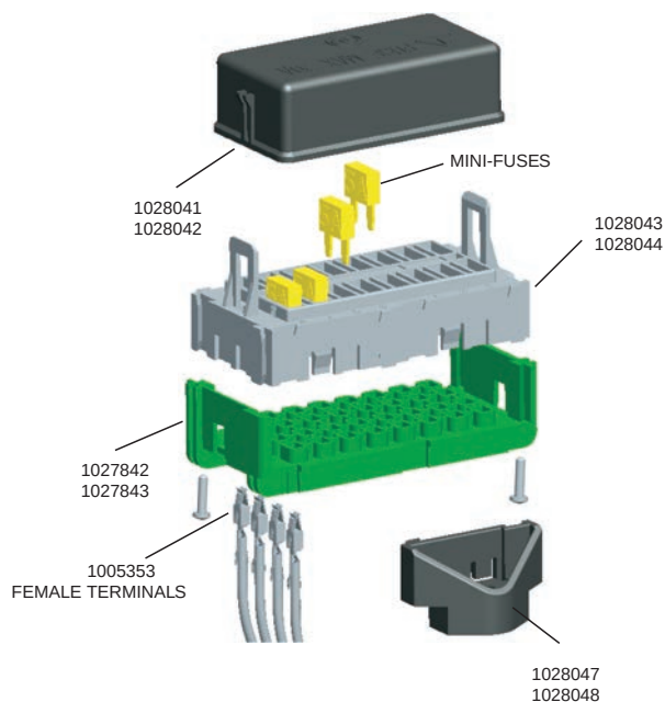
Coperchio Cover
