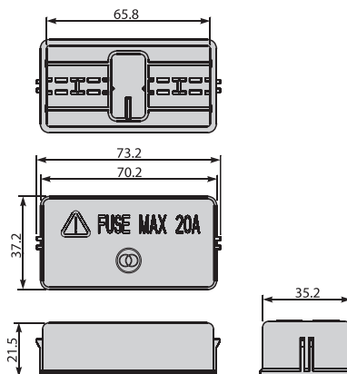
Coperchio Cover
