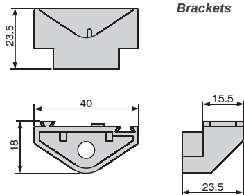
Staffe Brackets
