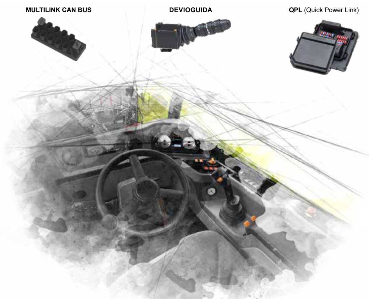
HMI (Human Machine Interface) DEVICES
